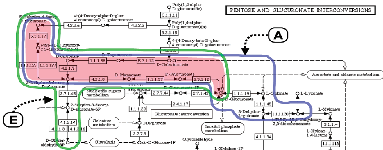
Figure 8. Example of the correlation between chemical information and genomic information. The area designated by A corresponds to the cluster of similar compounds shown in Figure 7. The area designated by E corresponds to the cluster of genomic associations where genes coding for the enzymes are closely located on selected genomes according to the KEGG ortholog group table. Thus, the shaded area is the overlap of chemical and genomic clusters.
