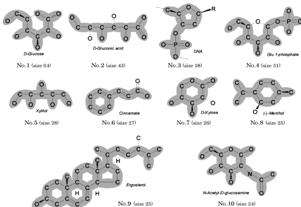
Figure 6. Common structures of the top 10 largest clusters. For each cluster a most representative compound is shown with its name, and the common structure is indicated in gray. The cluster size is shown in parentheses. The clusters 1, 2, 4, and 10 belong to the group of hexoses and derivatives, and their common structures are very similar. In fact, the four representative chemical compounds in this figure have high similarity scores each other. Apparently, the complete linkage method makes these clusters separated at the threshold score of 0.723, as well as the pentose-related clusters 5 and 7.
